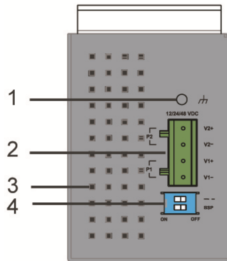
Rear Panel View
