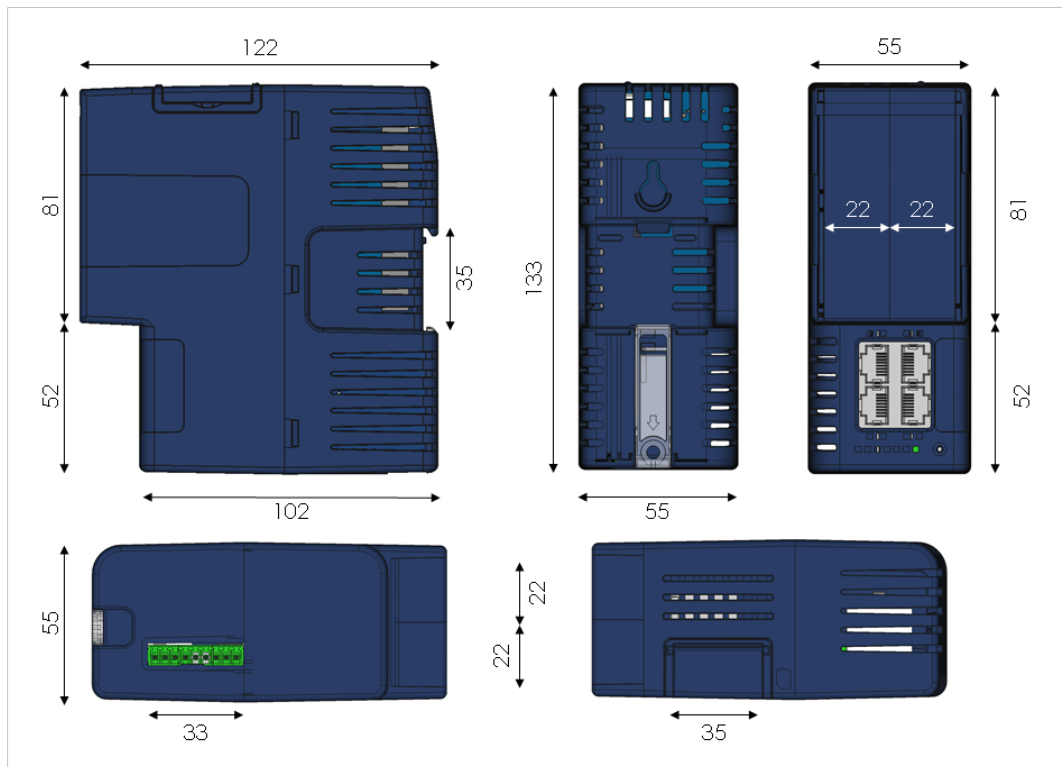
Fig. 7 Mechanical Dimensions
