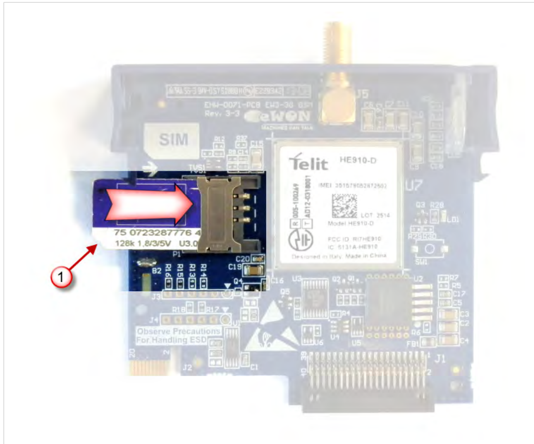
Fig. 6 SIM location on the FLB 3205
