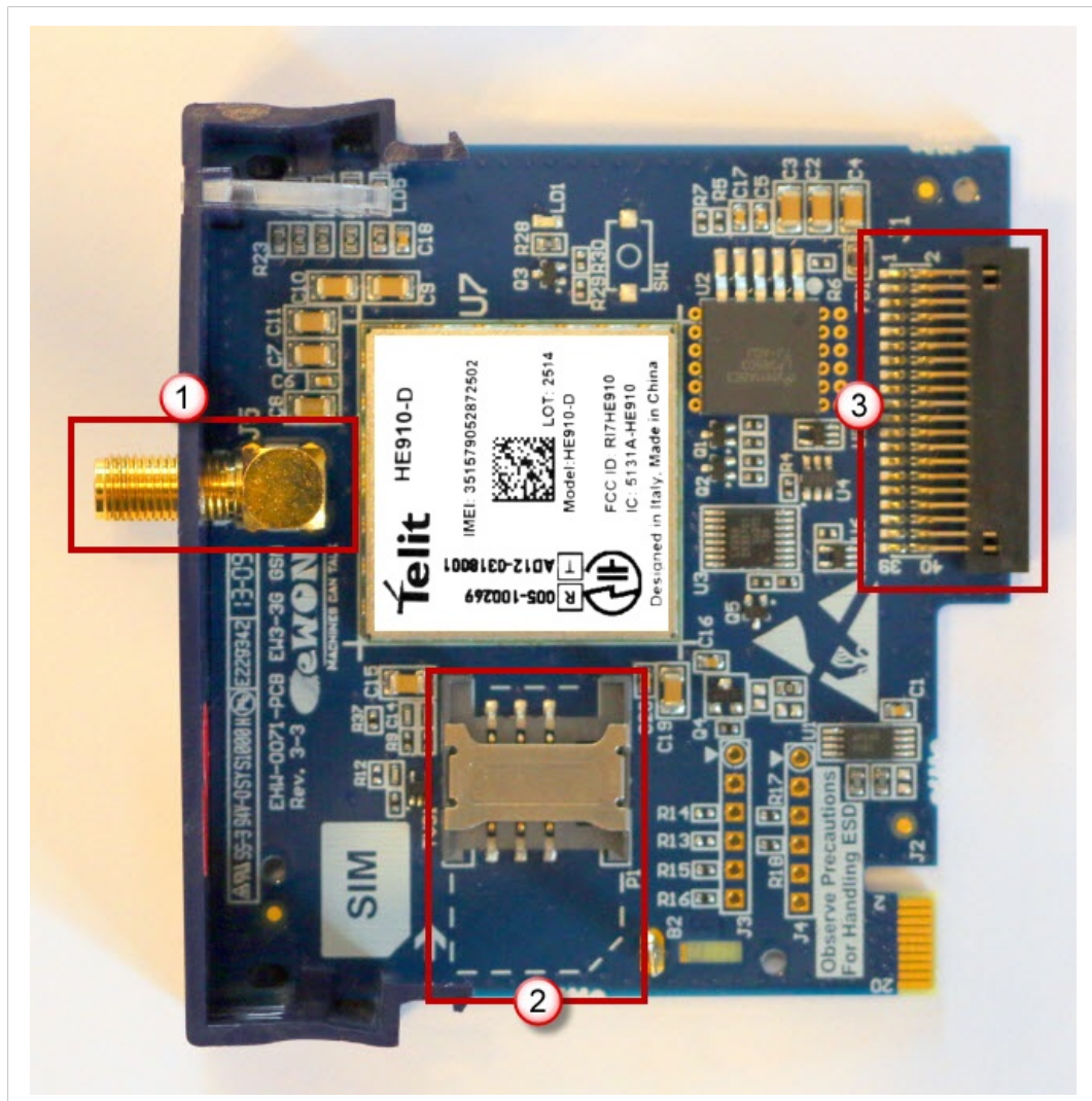
Fig. 1 Mechanical layout and interfaces
